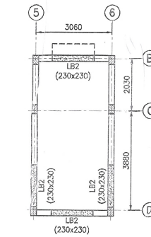
TERRACE FLOOR LINTEL BEAM LAYOUT (SCALE 1:100)
