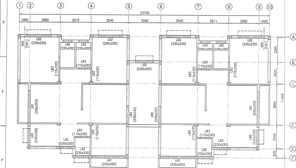
FIRST FLOOR LINTEL BEAM LAYOUT (SCALE 1:100)
