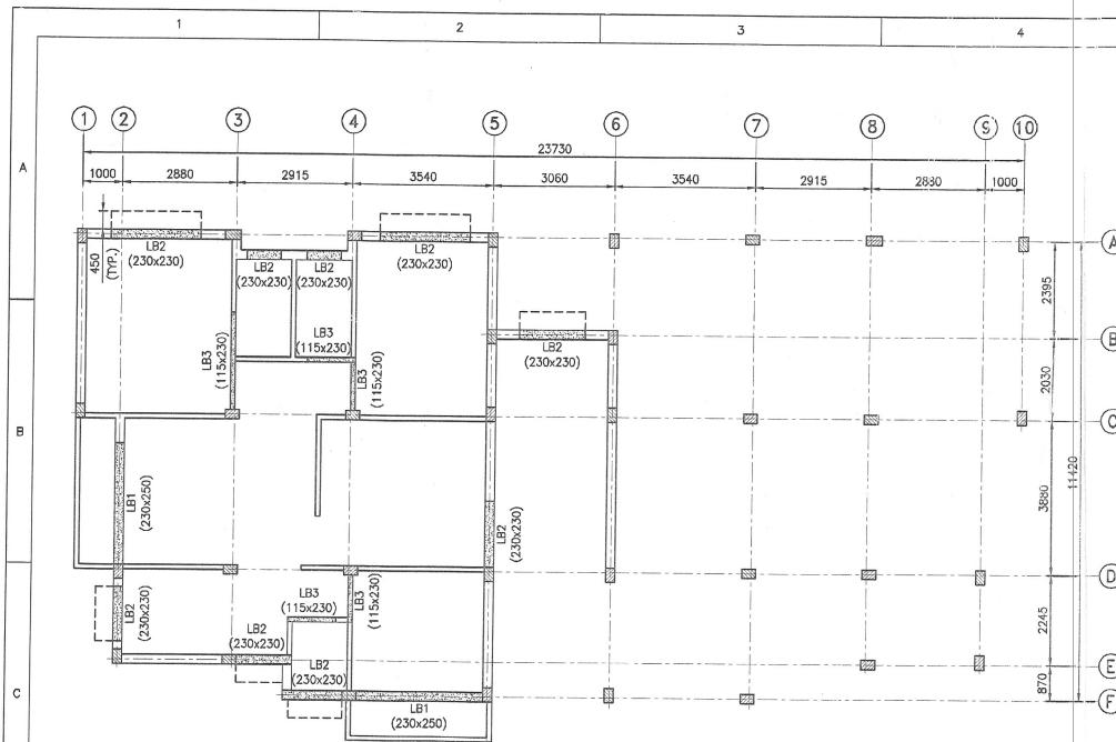
GROUND FLOOR LINTEL BEAM LAYOUT (SCALE 1:100)
