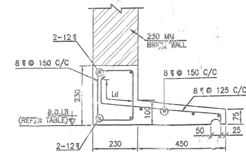
TYPICAL SEC. DETAIL OF SUN SHADE
