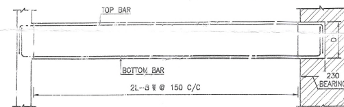
TYPICAL LONGITUDINAL SECTION FOR LINTELS (ONE SIDE COLUMN SUPPORT & OTHER SIDE BRICK WALL SUPPORT)
